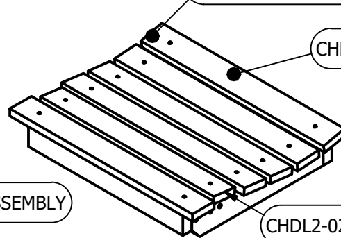
CHDL2-ASM-011 SEAT ASSEMBLY
